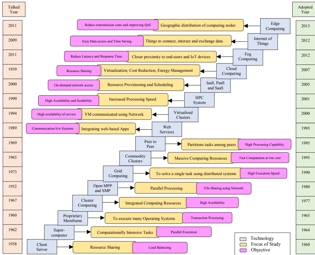
Figure 1: Evolution of Computing Paradigms and Technologies
